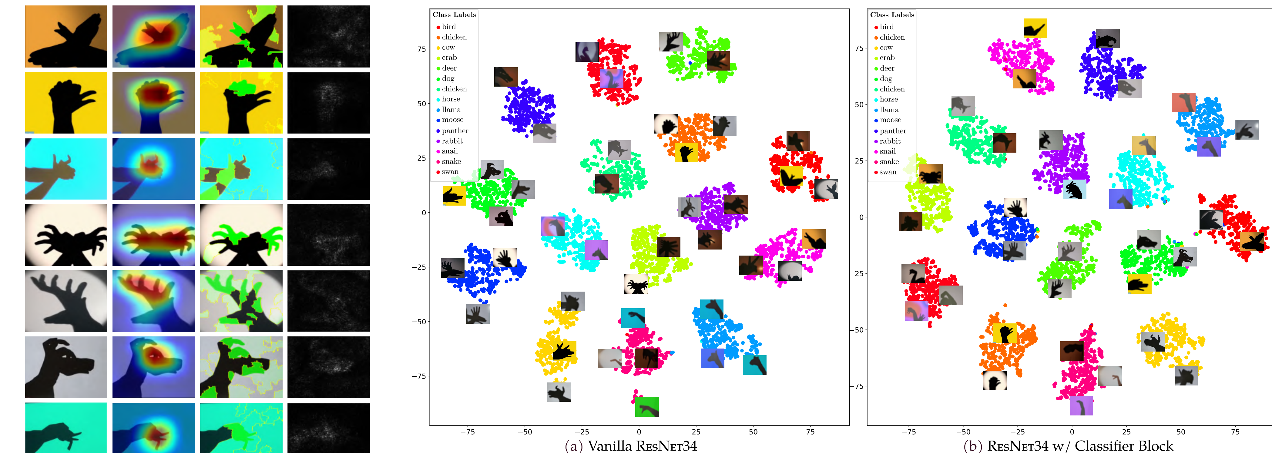
Figure 12. t-Distributed Stochastic Neighbor Embedding (t-SNE) feature representations of ResNet34
