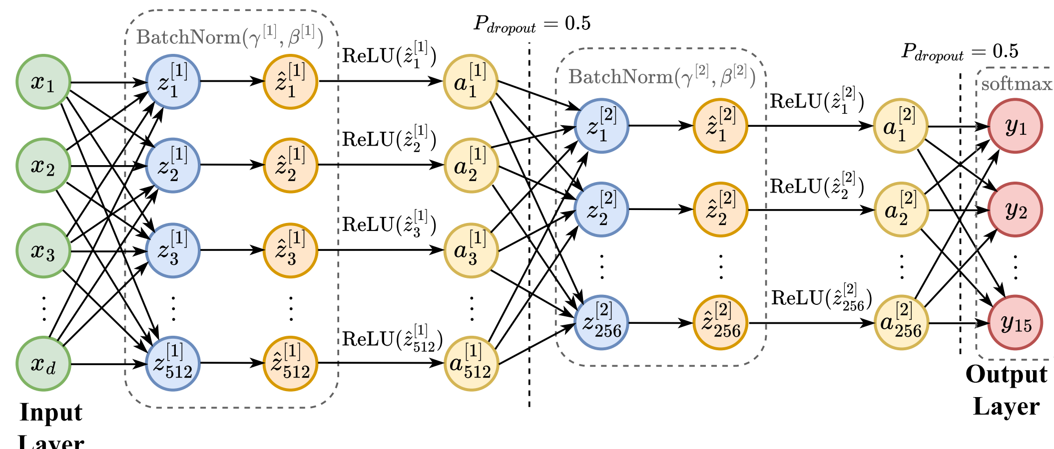
Figure 8. Classifier block attached to the tail-end of the pretrained models.
