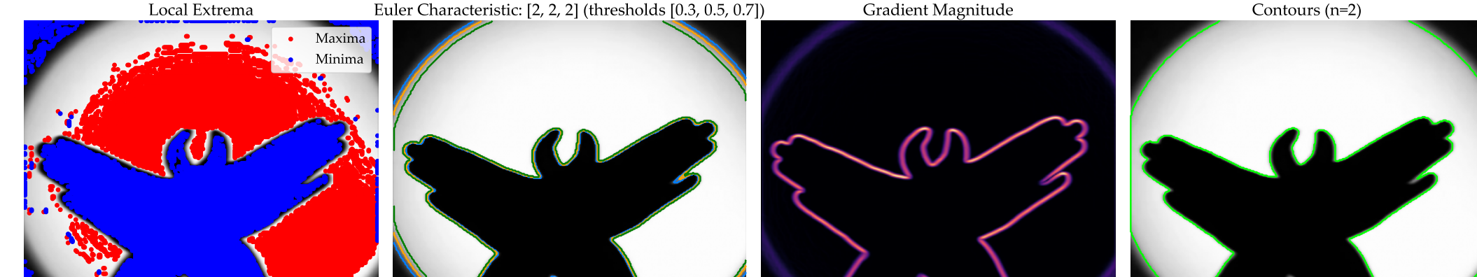
Figure 10. Topological features for a hand shadow puppet silhouette.
