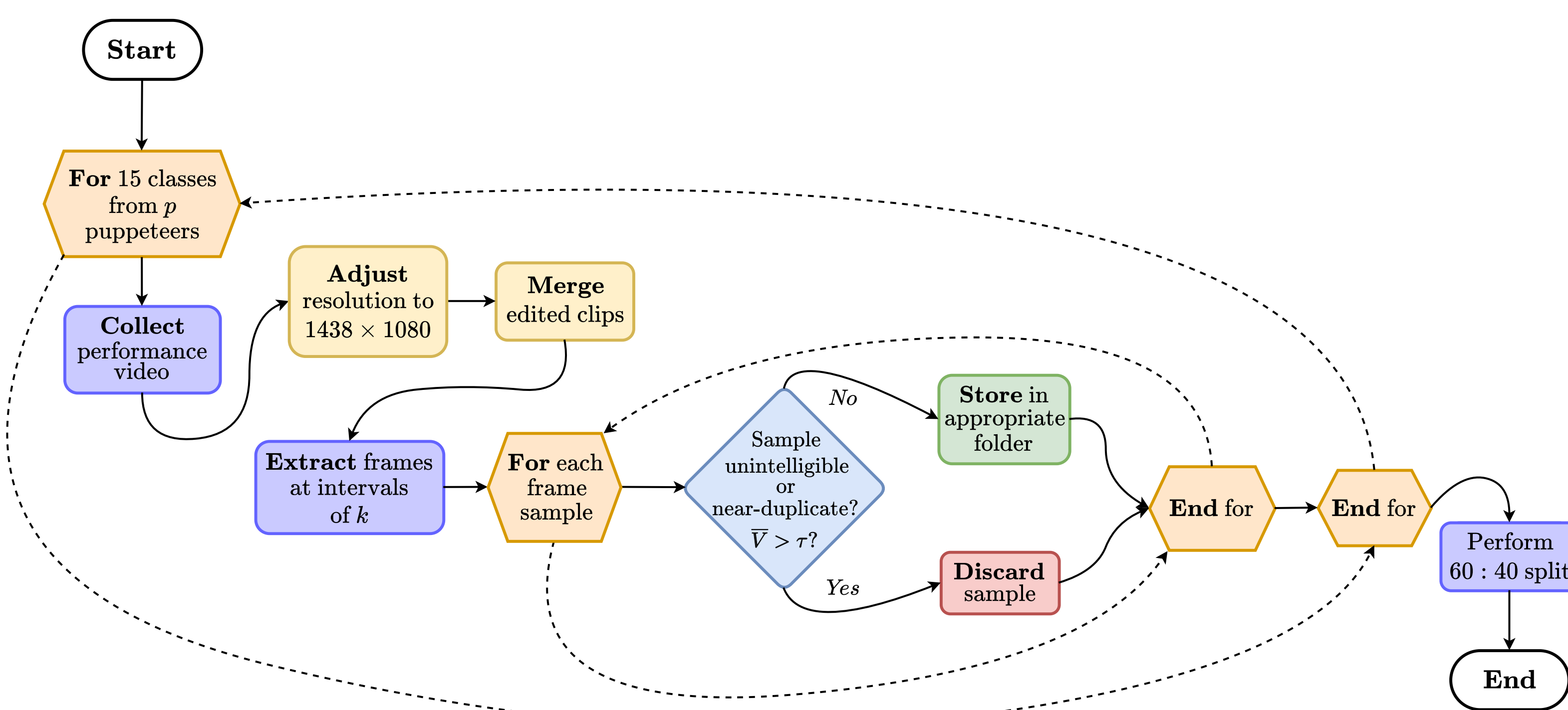
Figure 2. A flowchart depicting the dataset construction process.
