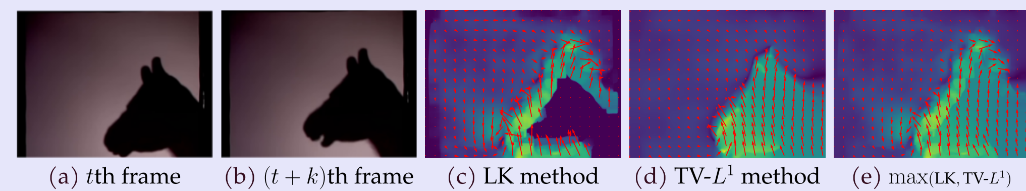
Figure 4. Optical flow estimation of contiguous candidate frames from the ‘Horse’ class.
